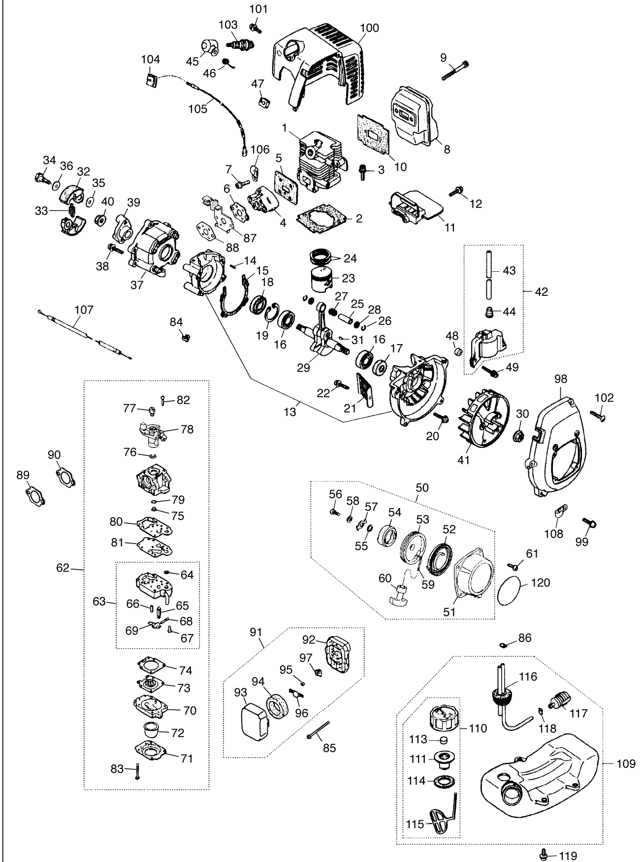
Fig. 4 ENGINE GROUP CHT2300B
