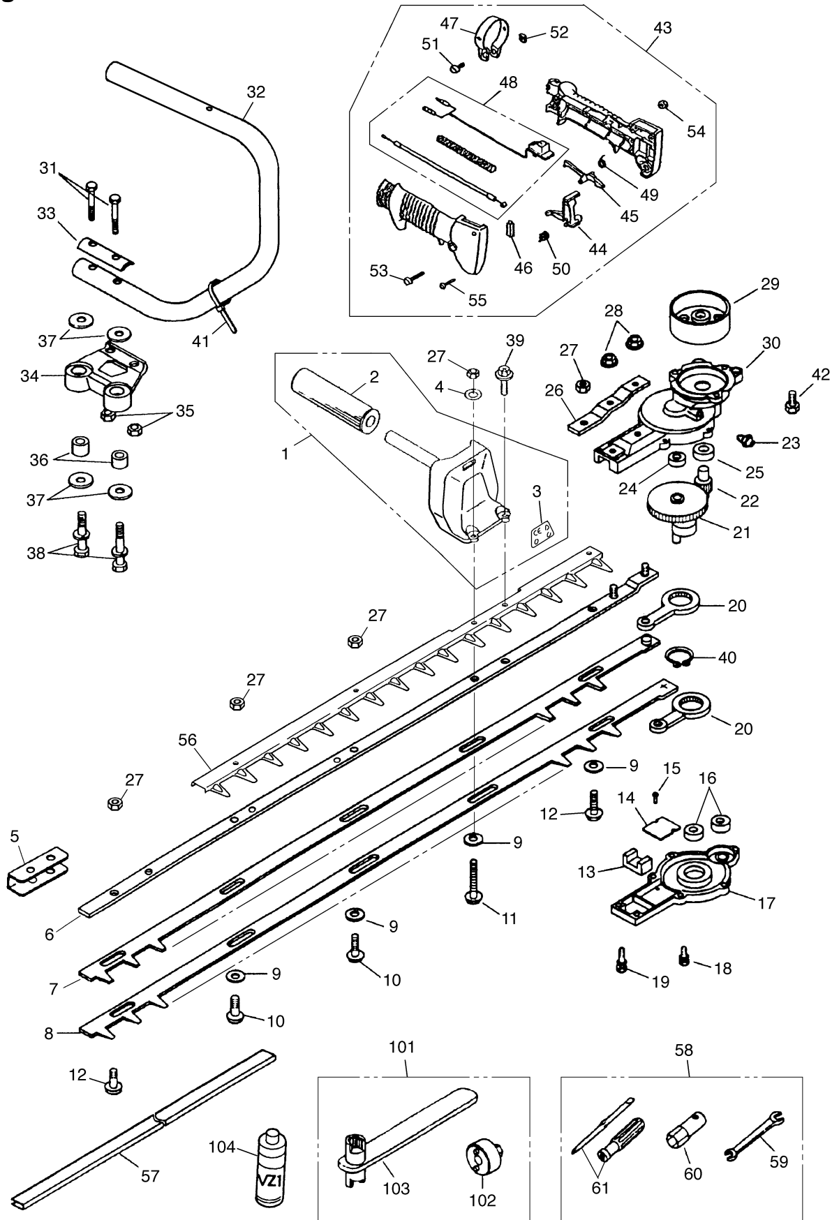
Fig. 1 CUTTER GROUP HT2300A
