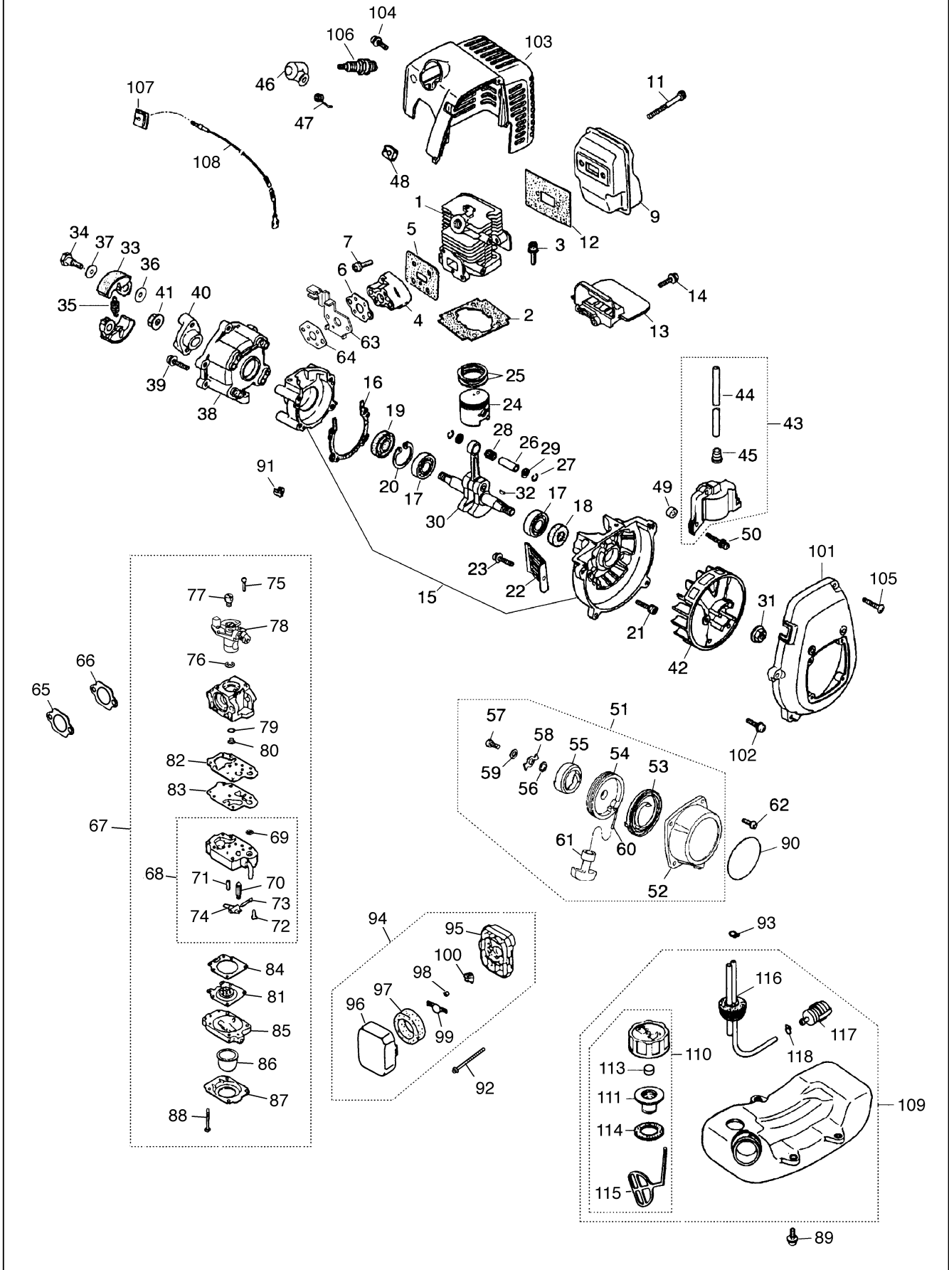
Fig. 2 ENGINE GROUP HT2300A
